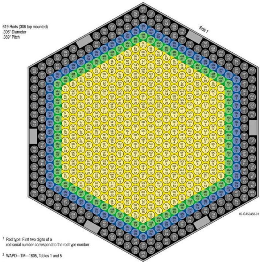
Figure 3-6. Light Water Breeder Reactor movable seed module rod arrangement and cell identification (modified from Figure A-1 of Gorscak, Campbell, and Clayton 1987, WAPD-TM-1605).
